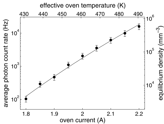
Fig. 8 The atom density from a collimated ytterbium beam with natural isotope abundance as a function of oven heating current. The beam is collimated by an aperture separated 3 mm from the oven nozzle. The density was measured approximately 5 mm away from the collimating aperture
