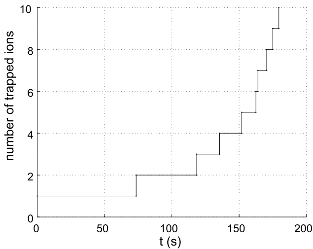
Fig. 14 Deterministic loading of a desired number of ions by two-color photoionization [1]. The loading rate increases with time, since the oven emitting YbI atoms heats up during the measurement
