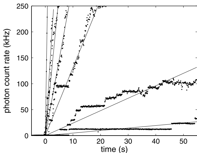
Fig. 10 Two-color photoionization of ^{172}\text{YbI} as a function of time for different electric currents heating the atom oven. The fluorescence signal is proportional to the number of trapped YbII ions for a low number of ions, i.e. short loading times (here, a single ion produces a photon count rate of \approx 15 kHz). In this region the signals are fitted by a linear function to extract loading rates as a function of oven current. Steps in the photon count rate for small heating currents indicate an increase by one of the number of trapped ions. The oven currents were (in order of ascending signal slope): 1.8 A, 1.9 A, 2.0 A, 2.18 A, 2.3 A, 2.47 A, 2.57 A
