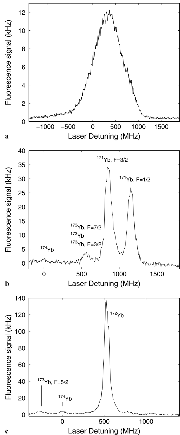
Fig. 3 Laser induced resonance fluorescence spectra of the ^1S_0-^1P_1 transition in YbI. An isotopically enriched sample of ^{171}\text{YbI} (a, b) or ^{172}\text{YbI} (c) was used. The detuning of the laser frequency is given relative to the resonance of ^{174}\text{YbI} . (a) ^{171}\text{YbI} : the angle between the laser beam and the atomic beam is about 45^\circ . The resonance is shifted and broadened by the Doppler effect. (b) ^{171}\text{YbI} : the laser beam crosses the atomic beam at right angles allowing for resolution of the hyperfine structure. The rest abundance of ^{172}\text{YbI} can be seen as a small resonance peak to the left of the two prominent hyperfine resonances of ^{171}\text{YbI} . (c) ^{172}\text{YbI} : Doppler-reduced spectrum
