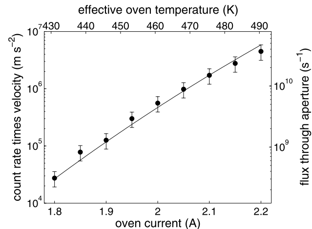
Fig. 9 The atomic flux density from a collimated ytterbium beam with natural isotope abundance as a function of oven heating current. The density data presented in Fig. 8 was combined with measurements of the line shift due to the mean beam velocity as shown in Fig. 3a
