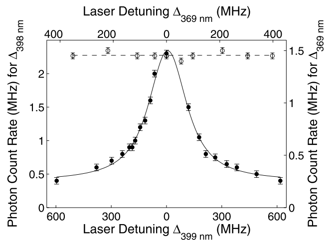
Fig. 13 Dependence of the ionic resonance fluorescence signal—and hence the loading rate—on detuning of both lasers for two-color photoionization during the loading time. The fluorescence signal shows a strong dependence on the detuning of the 399-nm laser ( filled dots ), since this excitation is a resonant process. The solid line indicates a fit using a Voigt profile. The non-resonant excitation with the 369-nm laser above ionization threshold shows no dependence on variation of wavelength ( open circles ) and can be fitted by a constant ( dashed line ). The ionization time was 30 s at 2.59-A oven current
