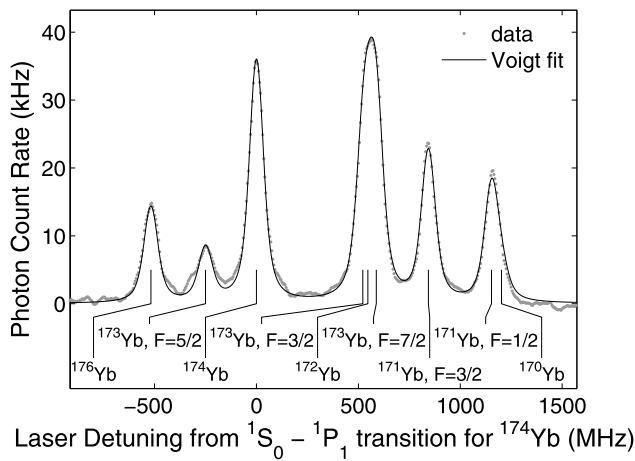
Fig. 4 Laser induced resonance fluorescence spectra of the ^1S_0-^1P_1 transition in YbI with reduced Doppler broadening from an oven with natural abundance isotope distribution. All hyperfine information displayed at the resonances concerns the upper levels of the transitions since the ground state exhibits no hyperfine splitting. Nonlinear regression was performed by assuming fixed spacing given by [35] and fitting a common horizontal and vertical displacement, a natural line width, a residual Doppler width, and individual peak heights
