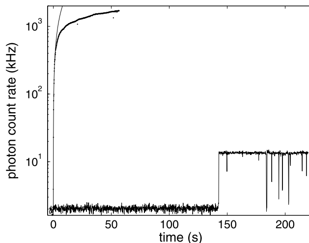
Fig. 11 Comparison of efficiency for electron impact and two-color ionization of ^{172}\text{YbI} (oven current set to 2.5 A) [1]. The upper trace (dots) shows the rise in fluorescence when two-color photoionization is used and a fit (solid line) to the linear slope of the signal as in Fig. 10 (note that the linear slope is not displayed as a straight line due to the logarithmic depiction). The step in the lower time trace (electron impact ionization) signifies the trapping of a single ion
