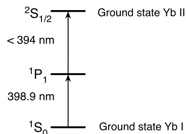
Fig. 2 Two-photon ionization of YbI via the ^1P_1 state
