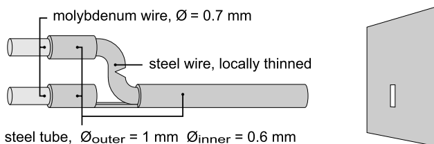
Fig. 5 Sketch of the oven
