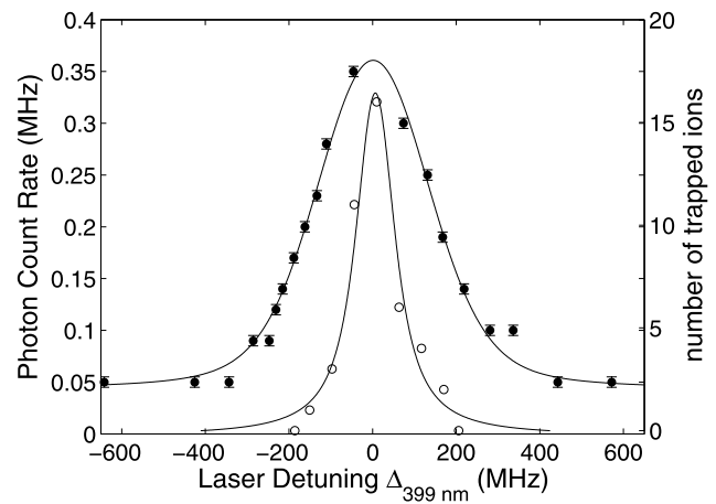
Fig. 15 Ionization efficiency of one-color photoionization of ^{172}\text{Yb} as a function of detuning of the 399-nm light from the ^1S_0-^1P_1 resonance. The filled circles show the fluorescence signal as a function of laser detuning, similar to Fig. 13. The ionization time was 30 s at an oven current of 2.59 A and laser and atomic beams enclose an angle of 45 degrees. Fitting a Voigt profile yields a FWHM of 320 MHz. The open circles display the number of trapped ions after a loading time interval of 30 s at 2.79-A oven current. Here laser and atomic beams are perpendicular yielding low Doppler broadening. Fitting a Voigt profile yields a FWHM of 110 MHz, which is consistent with fluorescence profiles from neutral ^{172}\text{Yb}
