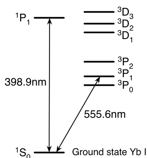
Fig. 2 Two-photon ionization of YbI via the ^1P_1 state
